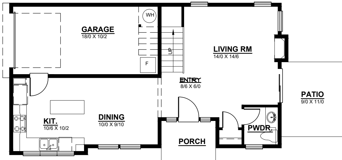
MAIN FLOOR PLAN - UNIT A/D
