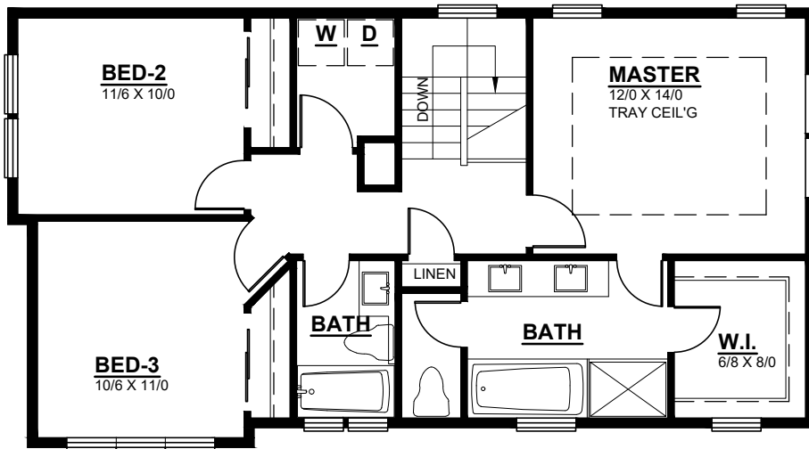
UPPER FLOOR PLAN - UNIT A/D
